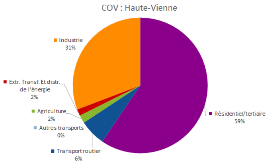
Figure 1 : Emissions COV - ICARE 2016 v3.2.2
