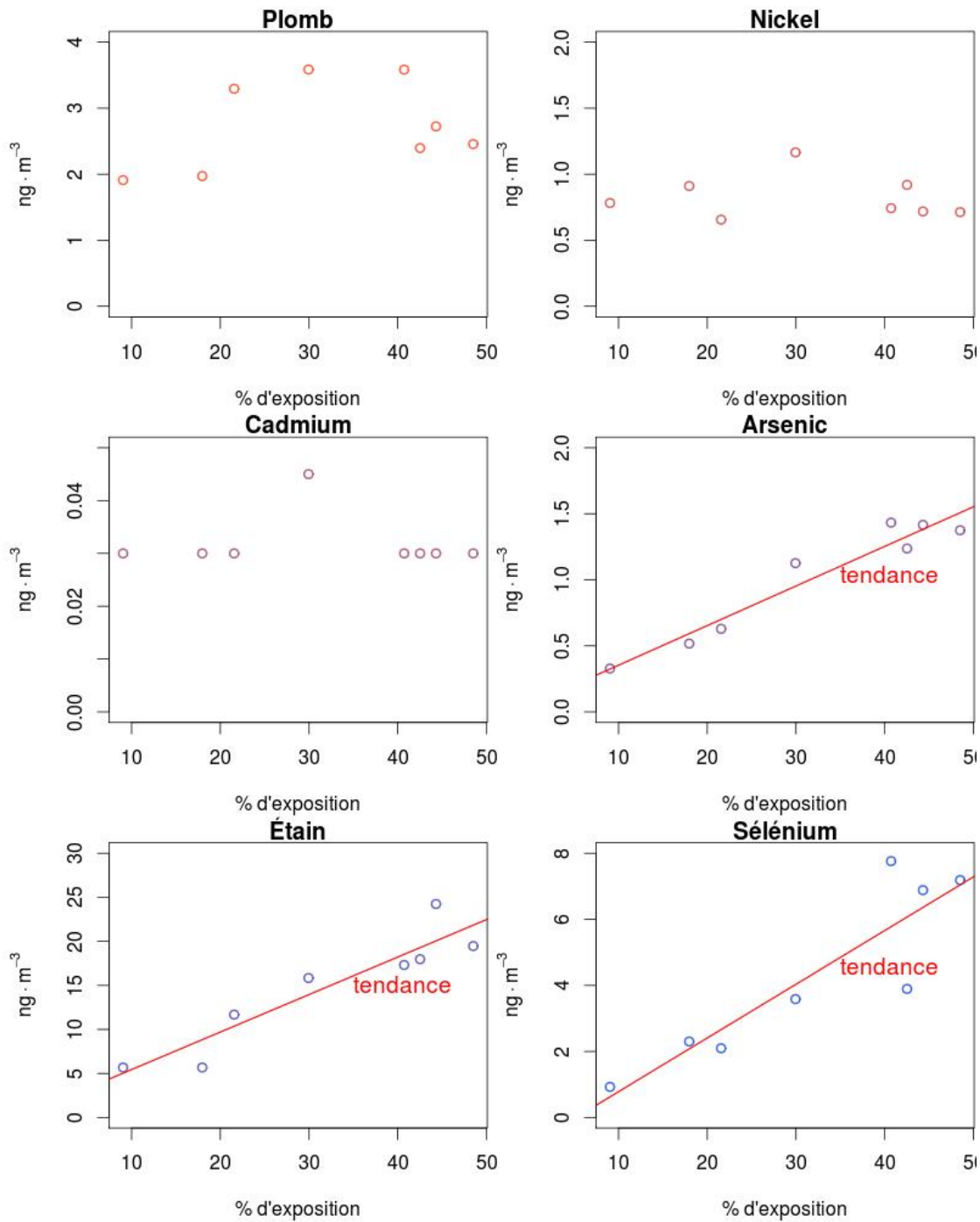
FIGURE 6.2 – Concentrations vs exposition, métaux lourds
